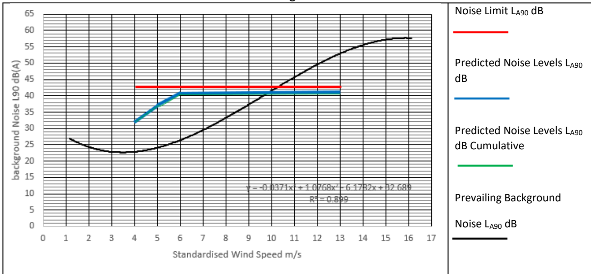
Location NM6 Night Noise Limit Curve
